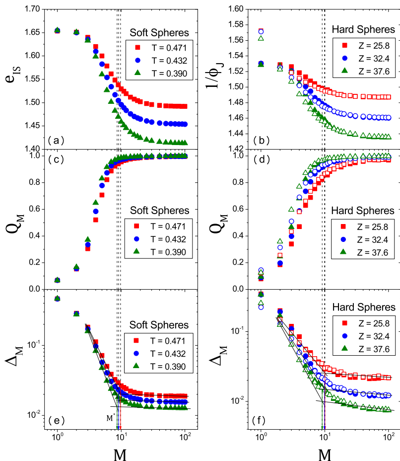
FIG. 3. ((a) and (b)) Inherent structure energy e_{IS} and volume 1/\phi_J . ((c) and (d)) Overlap Q_M . ((e) and (f)) Mean-squared displacements \Delta_M . The results are for additive soft spheres (left panels) and additive hard spheres (right panels) with \delta = 0.23 . The vertical dashed lines represents the M^* values determined by the intersection of the two power law regimes in the mean-squared displacements in (e) and (f). In addition to the “swap and quench” protocol with closed symbols, results for the “coarse-graining and quench” protocol are also shown for hard spheres using open symbols.
