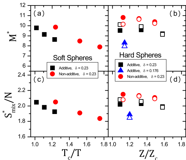
FIG. 4. Evolution of M^* for two soft sphere systems (a) and three hard sphere systems (b). (c) and (d) show the corresponding effective mixing entropy S_{mix}^* . The horizontal axes are normalized by the mode-coupling transition points, T_c and Z_c , to facilitate the comparison between the different models. In addition to the “swap and quench” protocol (closed symbols), results for the “coarse-graining and quench” protocol (open symbols) are also shown for hard spheres.
