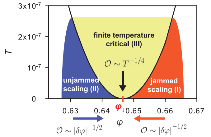
FIG. 9. The structure of the three scaling regimes where power law divergences and “anomalous” vibrational motion is observed. Regimes I and II are described by T = 0 harmonic theories, while dynamics in Regime III is fully anharmonic. These regimes are separated by the crossover temperature T^* \sim 10^{-3}(\varphi - \varphi_J)^2 discussed in Sec. VII. Note the small range of parameters where the effect of the T = 0 jamming critical point are felt and Eqs. (34) and (37) hold.
