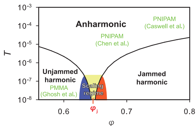
FIG. 13. An enlarged view of the (temperature, volume fraction) phase diagram reporting the critical regimes shown in Fig. 9, and the approximate location of the experimental studies aimed at studying anomalous vibrational dynamics in colloidal systems: Gosh et al. 10 use PMMA hard spheres, while Chen et al. 12 and Caswell et al. 16 study PNIPAM microgel particles. Previous studies all lie too far away from the jamming transition to detect the dynamic criticality associated to the transition.
