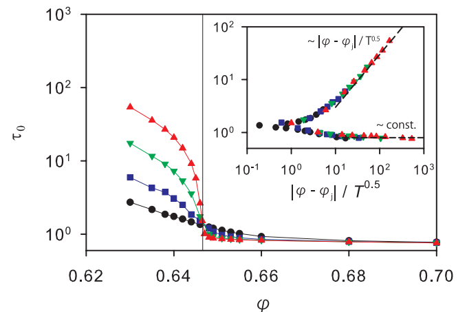
FIG. 3. Volume fraction dependence of the microscopic time scale \tau_0 , Eq. (8), at various temperatures decreasing from bottom to top using symbols as in Fig. 1. The vertical line indicates \varphi_J . These data were used to draw the open squares in Figs. 1 and 2. Inset: \tau_0 is replotted as a function of the scaling variable |\varphi - \varphi_J|/\sqrt{T} . Upper and lower dashed lines correspond to T \rightarrow 0 limits for hard and soft spheres, respectively, Eqs. (9) and (10).
