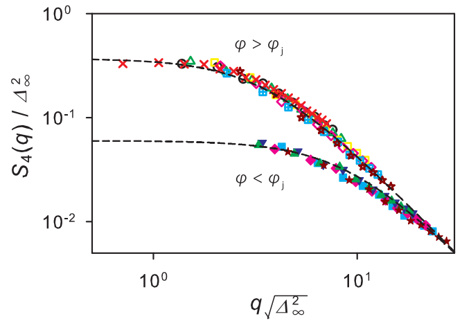
FIG. 7. Test of the scaling behavior of S_4(q) using the assumption that \xi_4 \sim \sqrt{\Delta_\infty^2} . Note that this data collapse involves no free parameter since S_4 and \Delta_\infty^2 result from independent measurements. Dashed lines are fits to the Ornstein-Zernike functional form, Eq. (28).
