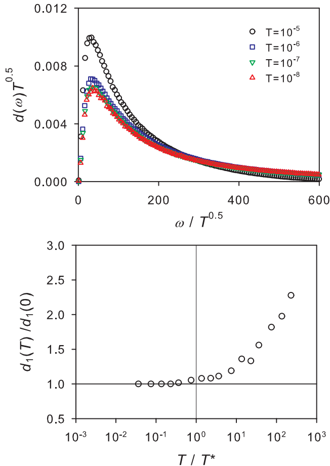
FIG. 10. Limit of validity of (effective) harmonic approximation below jamming. Top: Temperature-scaled density of state d(\omega)\sqrt{T} at \varphi = 0.630 and various temperatures converges to T = 0 limit below T^* \approx 10^{-7} . Bottom: Convergence of the height of the first peak of the DOS to its T = 0 value below the crossover temperature scale T^*(\varphi) = 10^{-3}(\varphi_J - \varphi)^2 . The vertical line indicates T/T^* = 1 .
