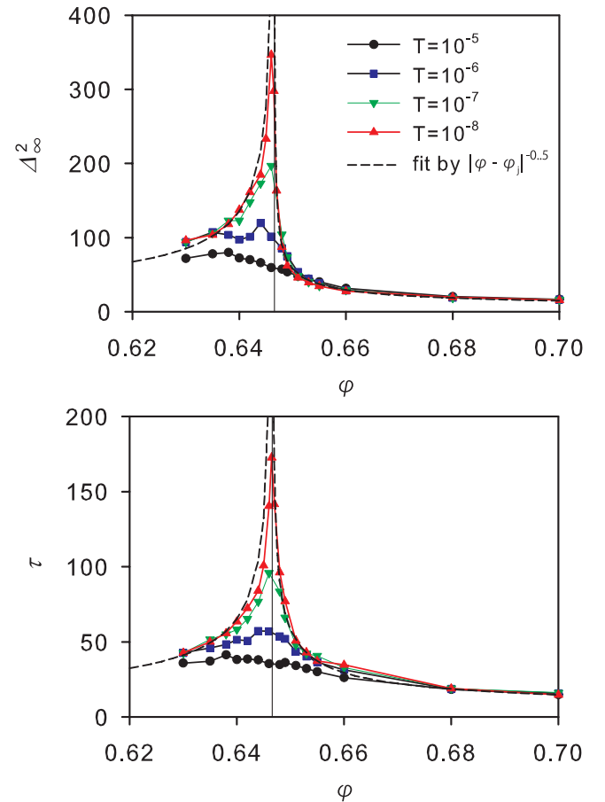
FIG. 4. Critical behavior for rescaled dynamic observables. Top: Rescaled Debye-Waller factor, Eq. (12). Bottom: Rescaled time scale for vibrational motion, Eq. (13). In both panels, dashed lines represent the critical divergence \sim |\varphi - \varphi_J|^{-1/2} , Eq. (18), and the vertical line indicates \varphi_J .
