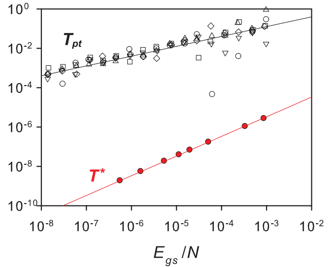
FIG. 11. The crossover temperature scale for the onset of anharmonicity T^* (bottom data with filled circles) compared to the temperature scale T_{\text{pt}} (top data with open symbols different symbols for different packings) quantifying the relevance of the high order terms in the perturbative expansion of the energy. The lines indicate T^* \propto E_{\text{gs}} and T_{\text{pt}} \propto E_{\text{gs}}^{1/2} . Clearly, these two temperature scales differ.
