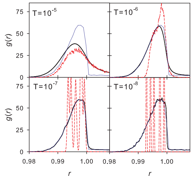
FIG. 12. The radial distribution function g(r) at finite T (black/thick lines), at T = 0 (blue/thin line), and its particle-resolved version g_i(r) (red/dashed lines) for a randomly chosen particle i at \varphi = 0.66 and various temperatures. While contacts between i and its neighbors are well-defined at low T , they cannot be resolved when T becomes larger than T^* which is \approx 4 \times 10^{-7} for this particular density.
