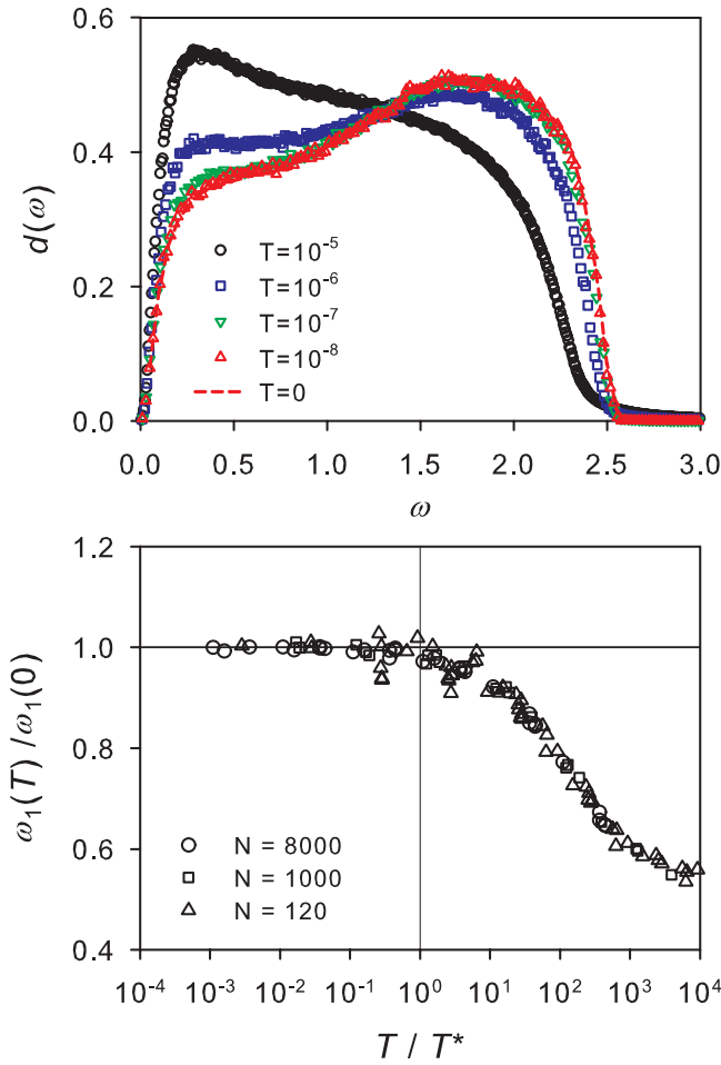
FIG. 8. Limit of validity of harmonic approximation above jamming. Top: The density of state d(\omega) at \varphi = 0.655 ( \varphi - \varphi_J \approx 0.0084 ) measured for various temperatures through Eq. (5). The T = 0 DOS is obtained from diagonalization of the dynamical matrix. Bottom: Convergence of the first moment of the density of state to its T = 0 limit below a crossover temperature scale T^* = 10^{-3}(\varphi - \varphi_J)^2 which is independent of system size. The vertical line indicates T/T^* = 1 .
