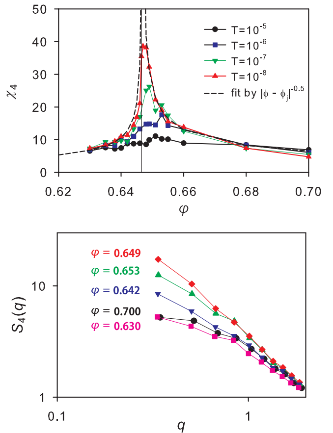
FIG. 6. Diverging susceptibility and length scale near the jamming transition. Top: Volume fraction dependence of the dynamic susceptibility \chi_4(t = t^*) , Eq. (22), for various temperatures showing the emergence of “vibrational heterogeneity” at low enough T close to \varphi_J (shown with the vertical line). Bottom: Four-point correlator S_4(q, t = t^*) at T = 10^{-8} and various volume fractions exhibits a nonmonotonic density dependence (note the nonmonotonic evolution of the \varphi labels).
