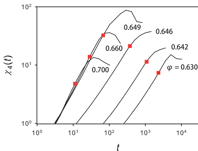
FIG. 5. Time dependence of the four-point susceptibility, Eq. (19), for T = 10^{-8} , and various volume fractions across \varphi_J . The filled squares indicate the timescale t^* . Note that \chi_4(t) saturates at long times to a system size dependent plateau.
