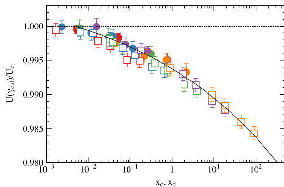
FIG. 5. The excellent collapse observed for U(\gamma_{c,d}, T)/U_e as a function of x_c = \gamma_c \tau_\alpha^b / T and x_d = \gamma_d \tau_\alpha^s / \sigma_0 for liquid-cooled films (squares), and vapor-deposited films (circles) indicates that surface relaxation plays the same role in the formation of vapor-deposited films as bulk relaxation in ordinary liquid-cooled film formation. Results are reported for temperatures T = 0.085 (red), T = 0.0825 (blue), T = 0.08 (green), T = 0.0775 (purple), and T = 0.075 (orange). The solid line is an empirical fit.
