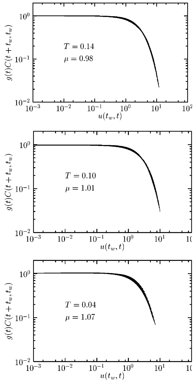
FIG. 13. Spin autocorrelation functions rescaled using Eqs. (23), (26), and (28). The temperature T and the exponent \mu are indicated in each figure.
