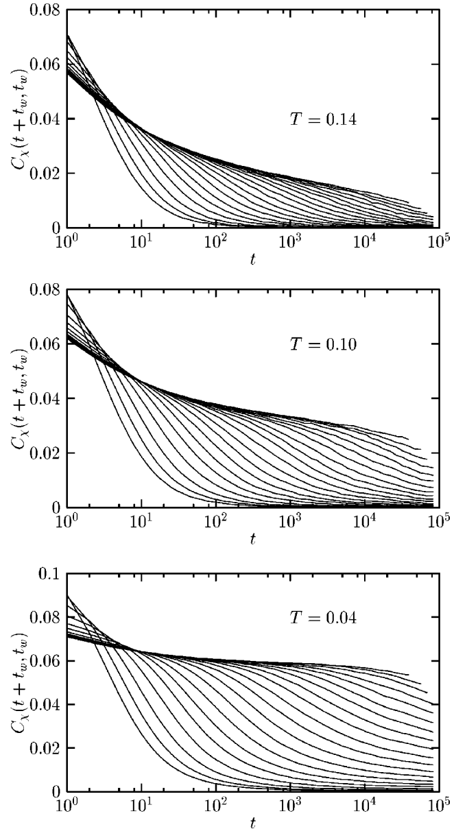
FIG. 4. Autocorrelation function of the chirality, Eq. (7), as a function of the time difference t for various waiting times t_w logarithmically spaced in the interval t_w \in [2, 5797] (from left to right). The temperature is T=0.14, 0.10, and 0.04 (from top to bottom).
